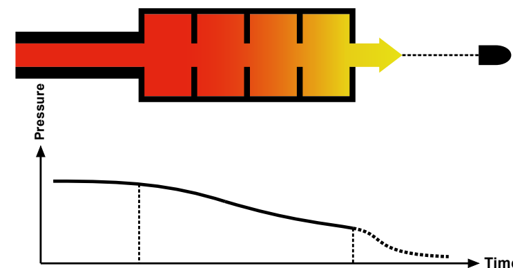
Conventional Suppressor
